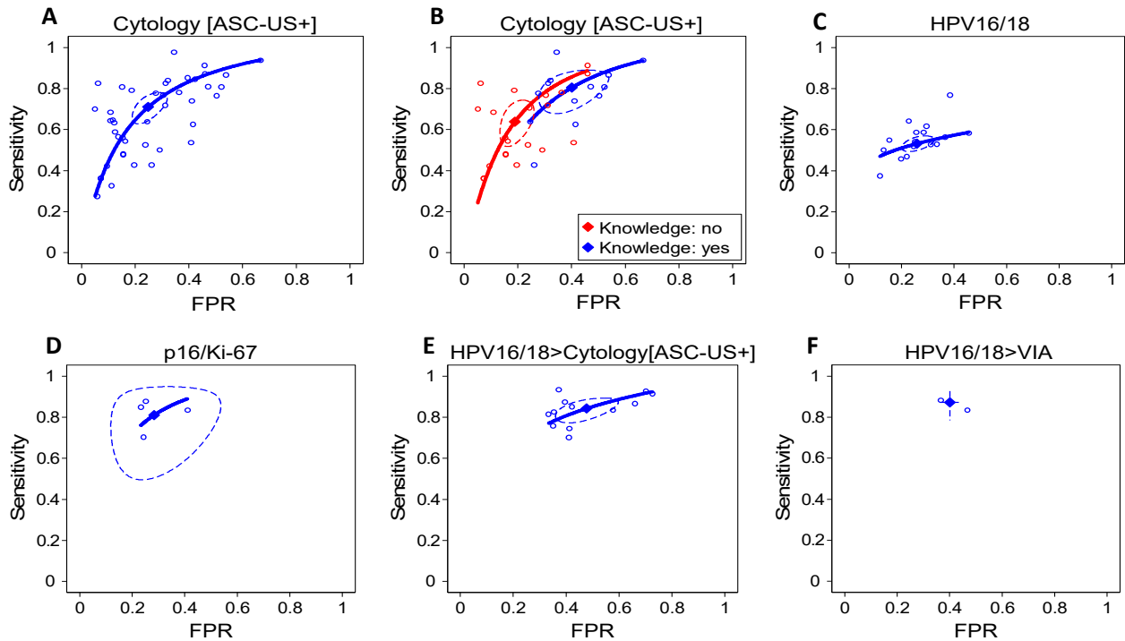
Fig. S4 Meta-analyses of the accuracy for detection of CIN2+ of six tests or combinations of tests used to triage hrHPV-positive women
